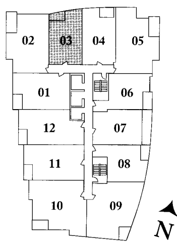
Typical Floor
